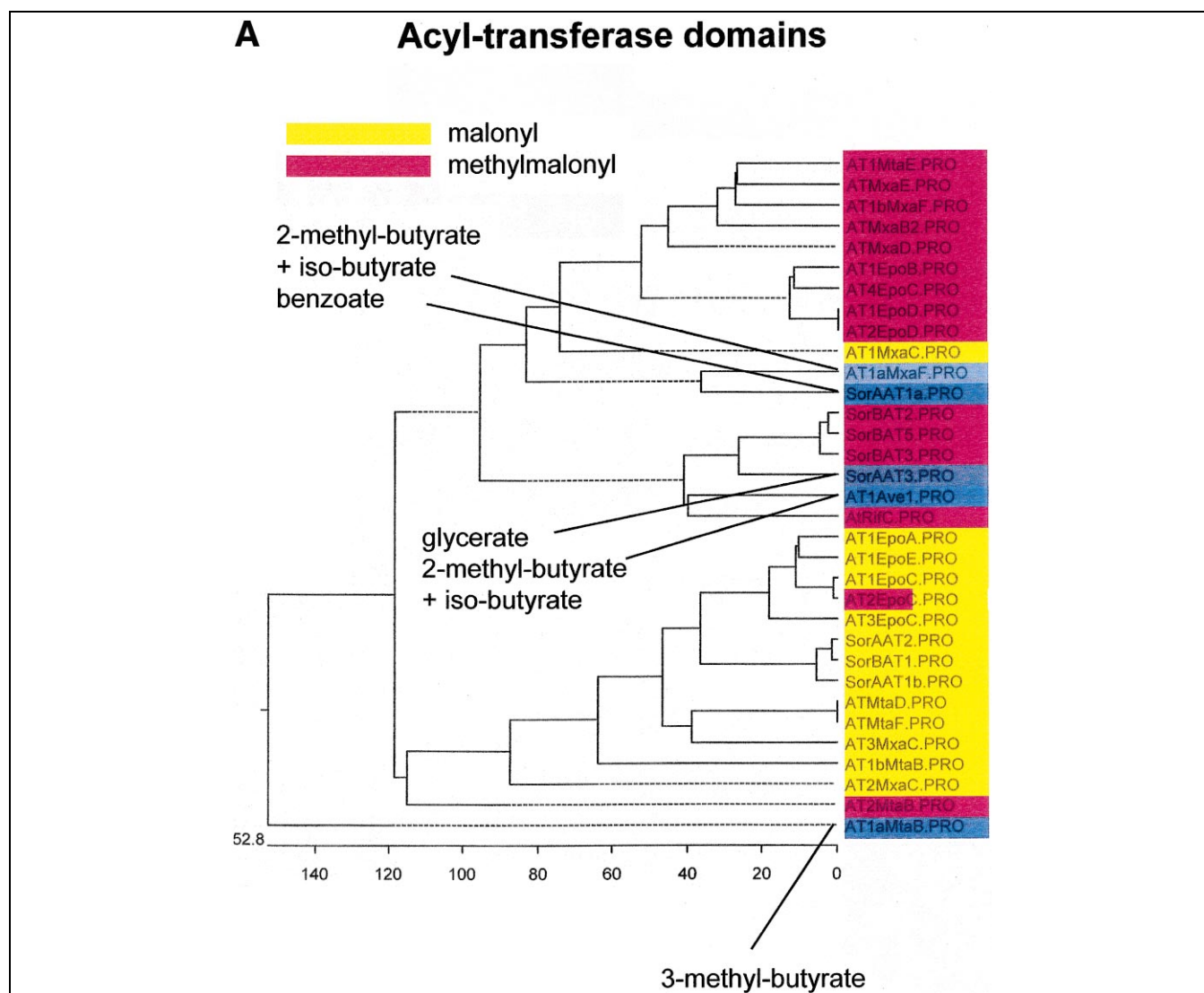
Fig. 5. Acyl-transferase domain alignment. A: Dendrogram of AT sequences from the epothilone (Epo; ref. see text), soraphen (Sor; ref. see text), myxothiazol (Mta; ref. see text), myxalamid (Mxa), avermectin (Ave; [31]) and rifamycin (Rif; [28]) biosynthetic proteins. Malonyl (m) and methylmalonyl (mm) specific ATs are shown in yellow and red, respectively. The ATs in blue are those with a different substrate specificity, which is referred to in the dendrogram. The length of each pair of branches represents the distance between sequence pairs, while the units at the bottom of the tree indicate the number of substitution events. A dotted line on a phenogram indicates a negative branch length. B: Alignment of the four AT domains discussed in the text. Boxes indicate the regions believed to determine substrate specificity [31], with the consensus sequence for each region given below the alignment. Amino acids in bold are those that are believed to specify malonate or methyl-malonate binding. Amino acids shown in red in the alignments do not fit into this hypothesis. Amino acids in green indicate the only differences between AT1 and AT2 of EpoC. '*' indicate identical, ':' similar aa.
